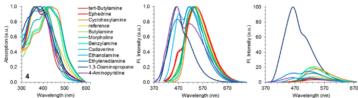
Figure 5. Absorption spectra (left), emission spectra (middle), and non-normalized emission spectra (right) of solutions of 4 in water/THF = 9:1 upon addition of different amines.
