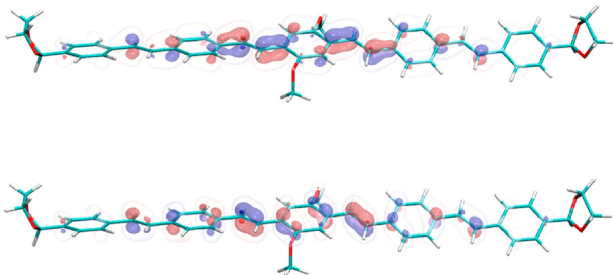
Figure 3. Highest occupied (HOMO, bottom) and lowest unoccupied molecular orbital (LUMO, top) of model compound 3m . The orbitals of the other model compounds are practically indistinguishable.
