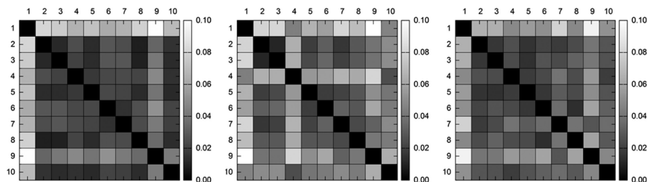
Figure 12. Autocorrelation plot (RAW rg values) of fluorescent dyes 1 , 4 , 13 , 16 , and 17 on neutral alox (left), silica gel (middle), and reversed phase silica gel (right) after exposure to amines recorded with a digital camera. When color information on identical amines + dyes are correlated the deviation \sigma_{nm} disappears (black squares on the diagonal).
