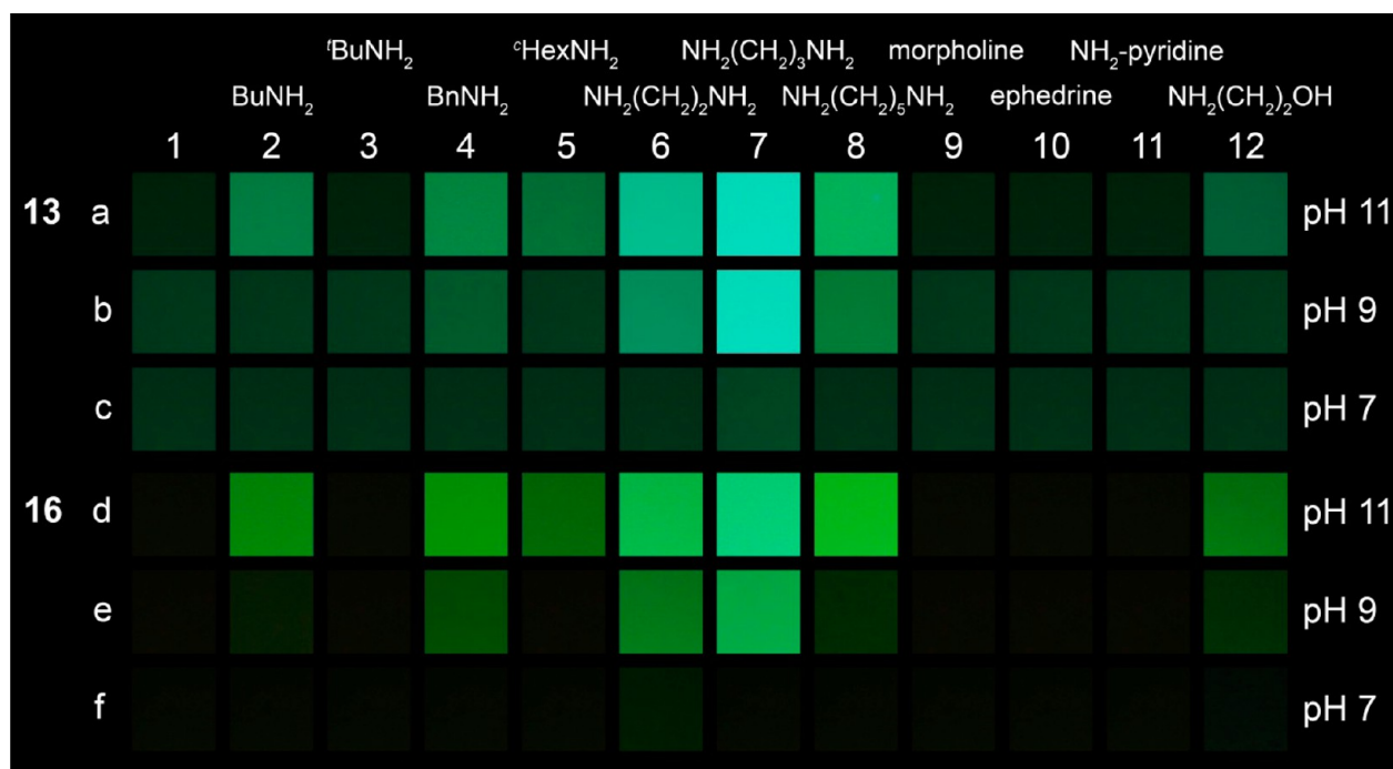
Figure 6. Photographs of buffered aqueous solutions ( c = 4.4 \mu\text{M} ) of 13 (a–c) and 16 (d–f) upon addition of amines 2–12 (left to right). Buffers: pH 11 (a, d), pH 9 (b, e), pH 7 (c, f). Columns: (1) fluorophore reference, (2) butylamine (10.43), (3) tert -butylamine (10.45), (4) benzylamine (9.34), (5) cyclohexylamine (10.64), (6) ethylenediamine (6.90/9.95), (7) 1,3-diaminopropane (8.49/10.47), (8) cadaverine (9.58/10.85), (9) morpholine (8.36), (10) ephedrine (10.14), (11) 4-aminopyridine (9.12), (12) ethanolamine (9.50). The samples were excited using a hand-held UV lamp at an emission wavelength of 365 nm. Photographs were taken with fixed settings of the camera (JPEG format, shutter speed 0.05 s, ISO value 100, aperture F2.8, white balance 6500 K, and Adobe RGB 1986 color space). The numbers in parentheses give the \text{pK}_a of the ammonium salts.
