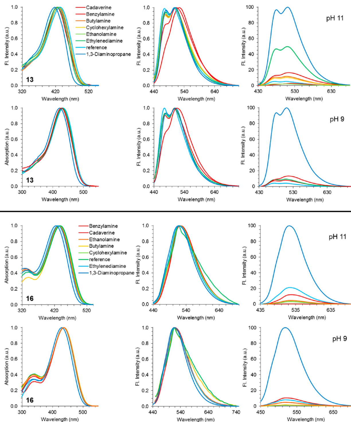
Figure 7. Absorption spectra (left), normalized emission spectra (middle), and non-normalized emission spectra (right) of buffered aqueous solutions (top: pH 11, bottom: pH 9) of 13 and 16 upon addition of different amines.
