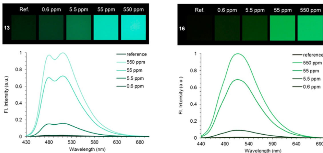
Figure 9. Photographs and fluorescence spectra of buffered aqueous solutions (pH 11, c = 4.4 \mu\text{M} ) of 13 (left) and 16 (right) at the concentrations of 1,3-diaminopropane specified in the panel.
