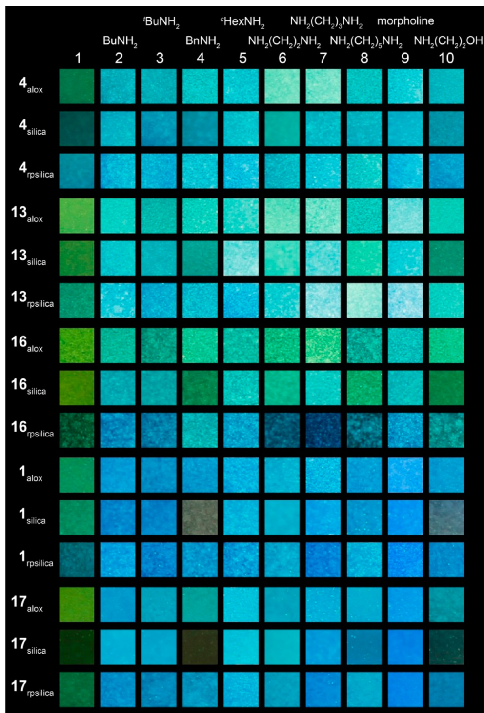
Figure 11. Photographs of samples of 4, 13, 16, 1, and 17 on alox, silica gel, and reversed phase silica gel TLC plates after 20 h of exposure to amine vapors 2–10 (left to right). Columns: (1) fluorophore reference, (2) butylamine, (3) tert -butylamine, (4) benzylamine, (5) cyclohexylamine, (6) ethylenediamine, (7) 1,3-diaminopropane, (8) cadaverine, (9) morpholine, (10) ethanolamine. The samples were illuminated using a hand-held UV lamp at an emission wavelength of 365 nm and photographs were taken with fixed settings of the camera (JPEG format, shutter speed 0.05 s, ISO value 100, aperture F2.8, white balance 6500 K, and Adobe RGB 1986 color space).
