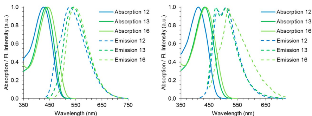
Figure 2. Absorption and emission spectra of 12 , 13 , and 16 in dichloromethane (left) and in water (right).
