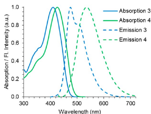
Figure 1. Absorption and emission spectra of 3 and 4 in dichloromethane.
