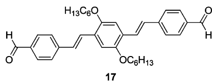
Figure 10. Structure of compound 17 .
