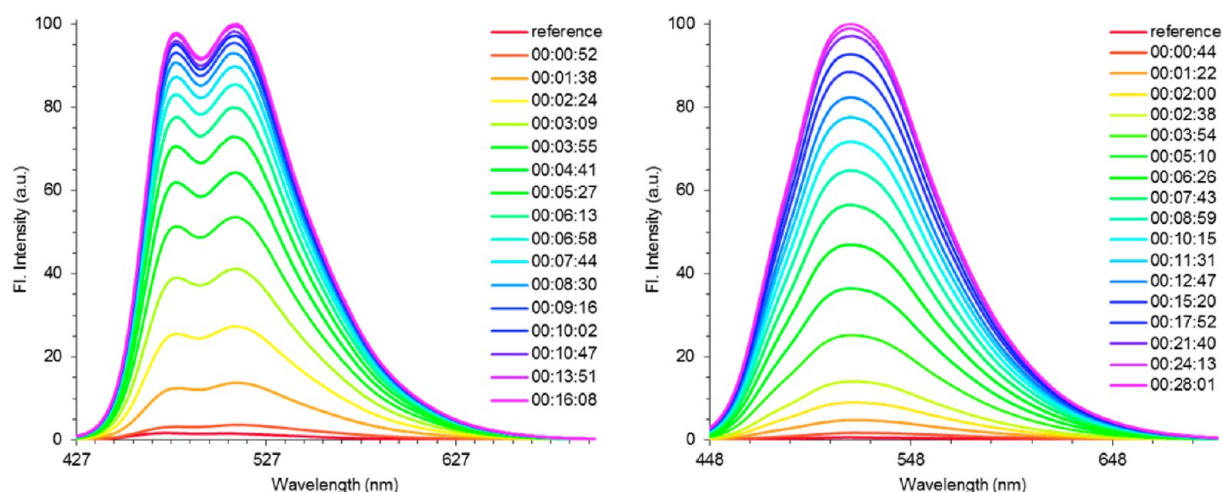
Figure 8. Time-dependent evolution of the emission wavelength and emission intensity for the reactions of 13 (left) and 16 (right) in a buffered aqueous solution (pH 11, c = 0.9 \mu\text{M} ) with 1,3-diaminopropane (120 ppm (vol)).
